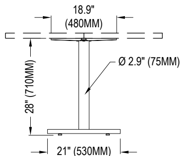
DINING ELEVATION
